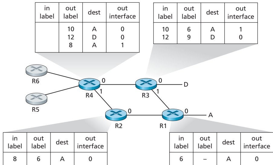
Figure 5.29 ♦ MPLS-enhanced forwarding
