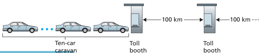
Figure 1.17 ♦ Caravan analogy
