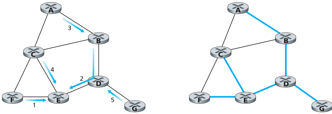
a. Stepwise construction of spanning tree
